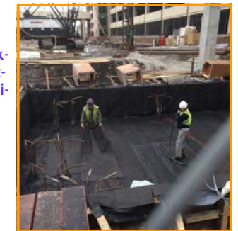
Installation of Waterproofing System with Geo-Seal™ and Bentonite Seal Layers
